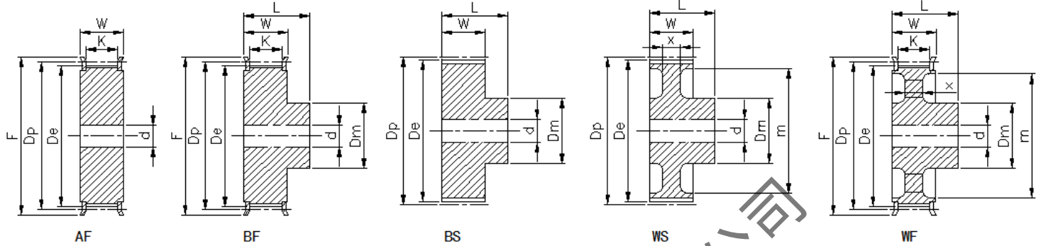
8M型同步带轮50mm
